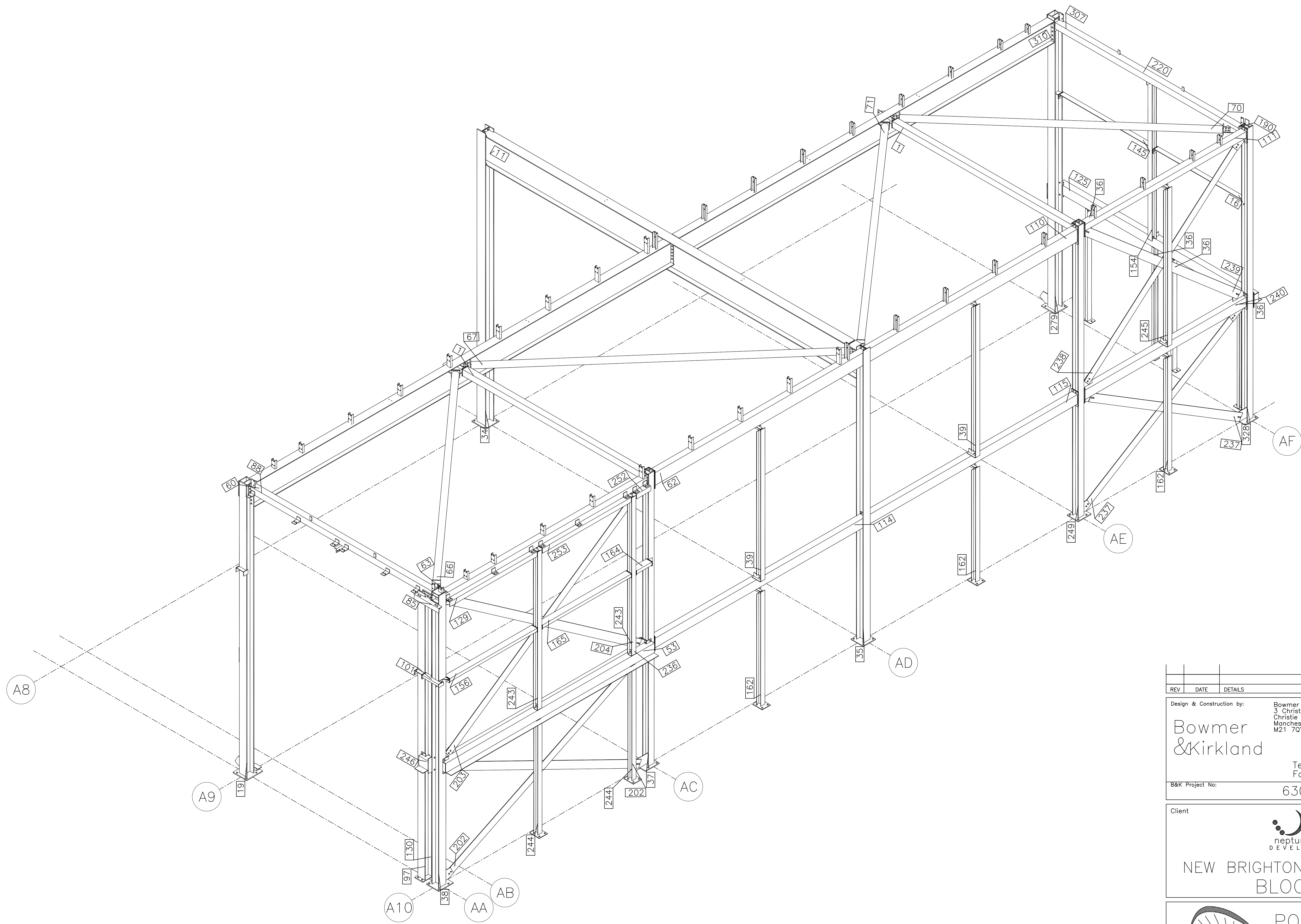
3-D MARKING VIEW LOT "1"
